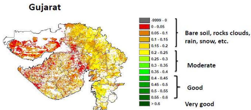
NOAA/VIIRS/BLENDED NDVI Composite ending on Week no 29 (16.07.2021 to 22.07.2021) over Agricultural region
